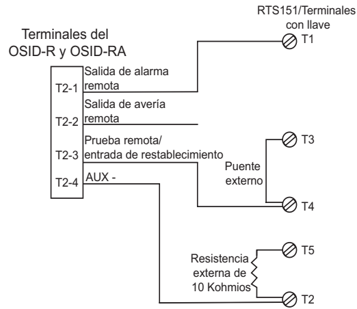
Figura 11-4: Diagrama de cableado (RTS451 o RTS151)
