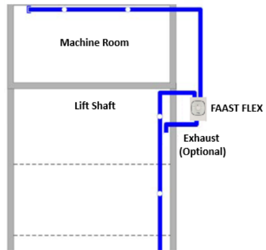
Figure 4: Machine Room / Shaft Protection
