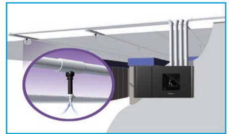
VESDA Pipe Network
