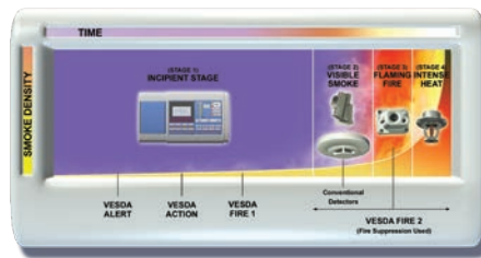
Figure 1 - Fire Growth Curve
