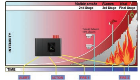
Fire Growth Curve
