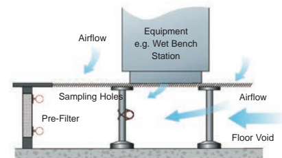
Sample pipe in the floor void beneath a raised access floor will capture smoke as it is carried by the airflow.
