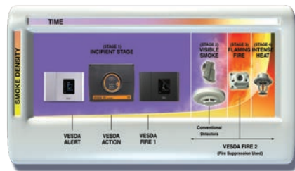
Figure 1. VESDA smoke detectors can be configured to detect a fire at the earliest stage. The multiple alarm levels can be configured to initiate an appropriate response.
