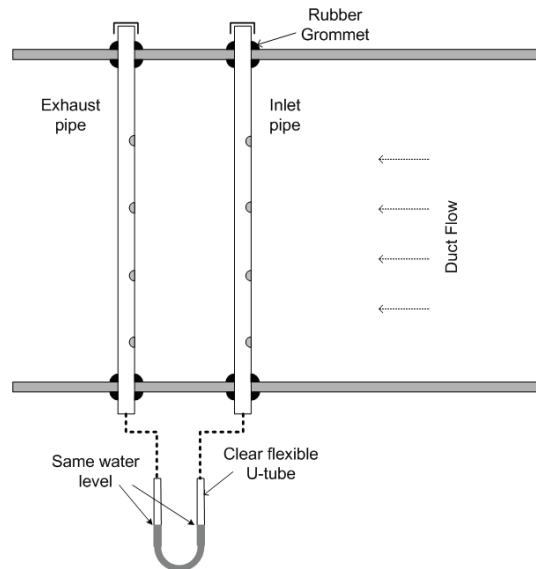
Figure 7 – Flexible U-tube set-up for hole orientation adjustment.
