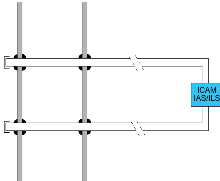
Figure 5 – Remote mounting
