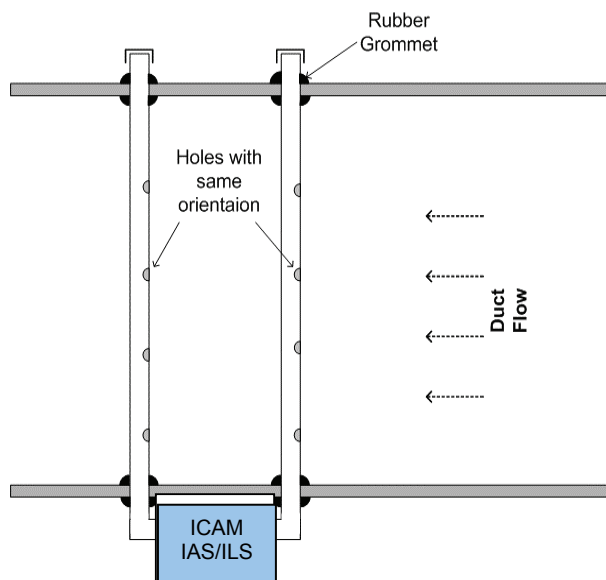
Figure 2 – Top view of the inlet and exhaust pipe positions, including sampling hole location, for a small duct.
